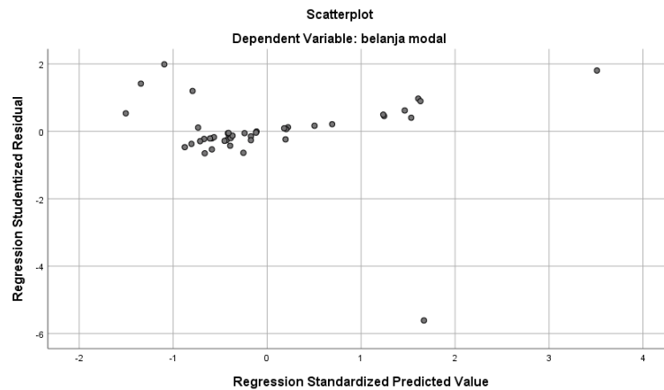
Gambar 4.2 Scatterplot
