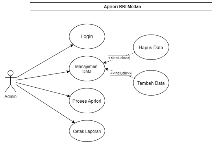
Gambar 4 Usecase Diagram Apriori RRI Medan
