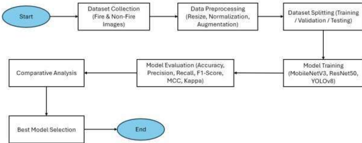
Fig. 1 Overall Research Workflow for Forest Fire Image Classification
